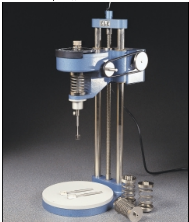
EL26-2270 Laboratory Vane Apparatus and Accessories
